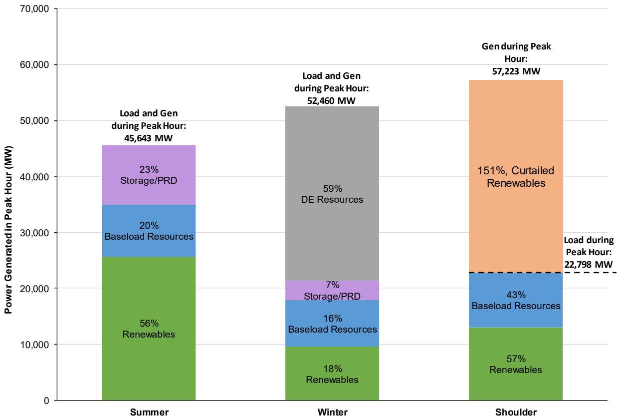
Figure 36: Resource Mix during Seasonal Peak Load Hours (CCP2-CLCPA Case)
