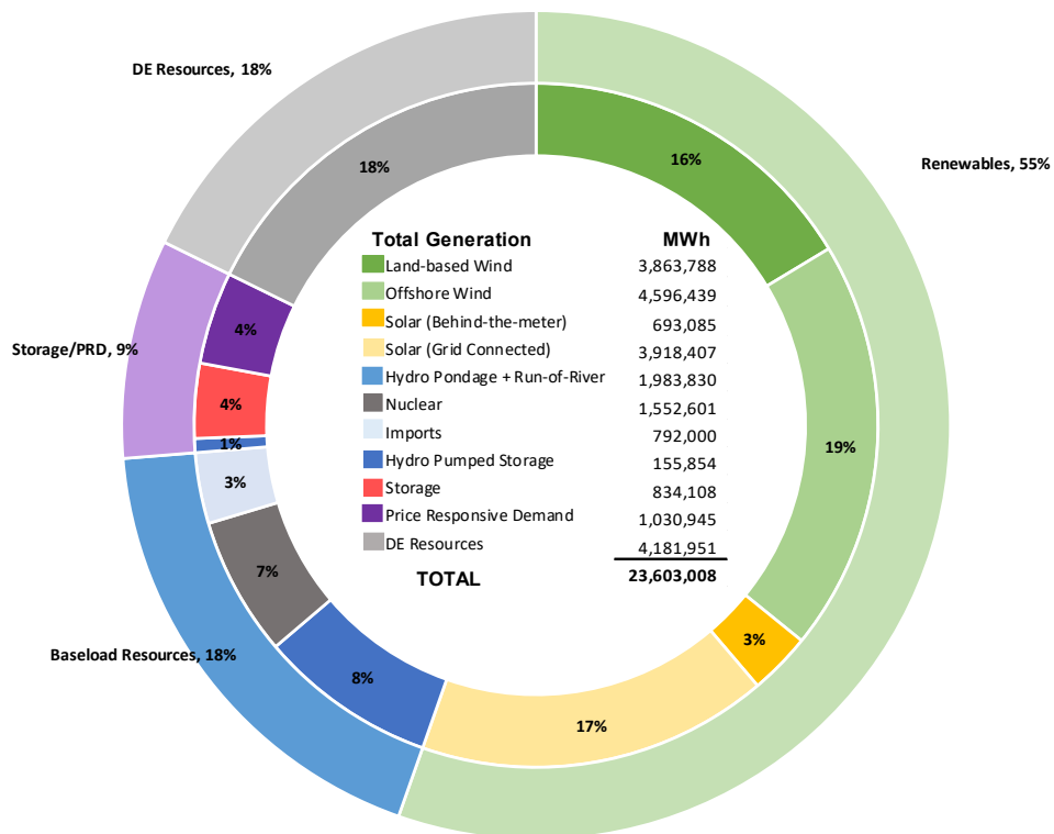
Figure 49: Summer Generation by Resource Type - CLCPA Case with Grid in Transition Resource Set
